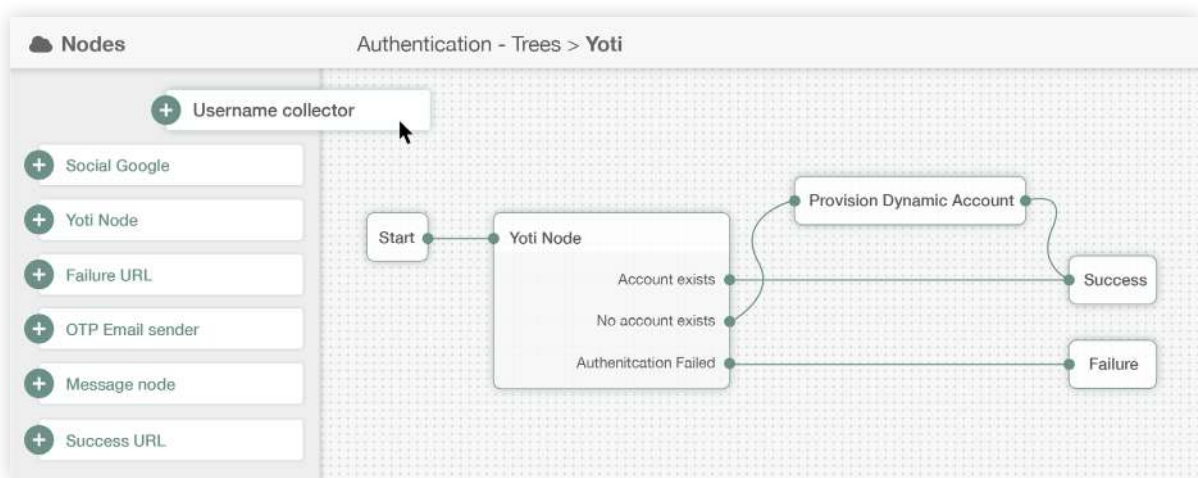
Building an authentication journey on the ForgeRock Access Management platform
